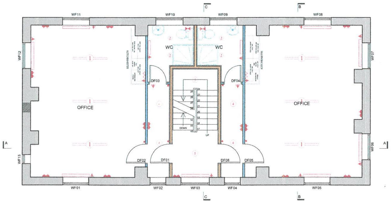
First Floor Plan (Area 95.25m 2 )
